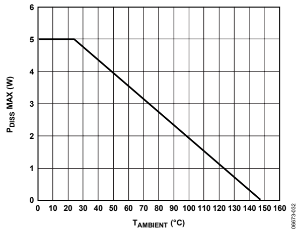
Figure 32. Power Dissipation Derating vs. Ambient Temperature
